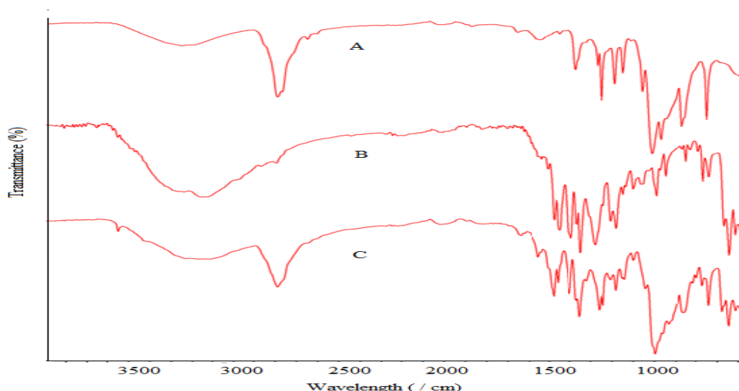
Figure 3: FTIR Spectrum of (A) PEG-VPB alloy, (B) Diclofenac sodium, (C) Batch C tablet
